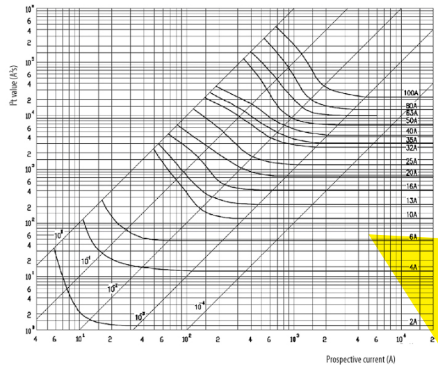
Melting energy characteristics Pt
