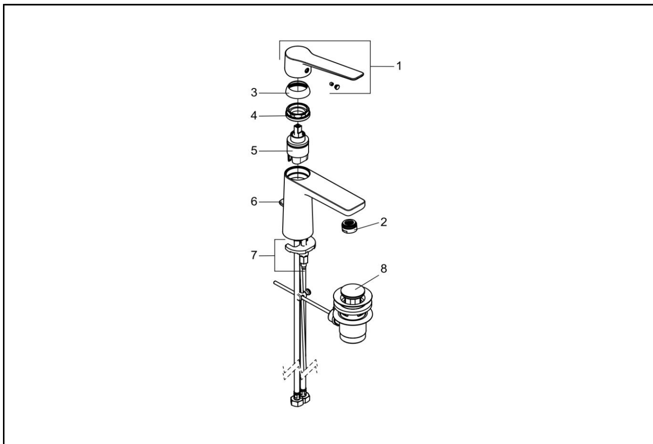
V3DEP Einhand-Waschtischbatterie derby V3 plus m. Hebel geschl. m. AG chrom VIGOUR Single-lever basin mixer derby V3 plus closed Lever with drain set chr. VIGOUR
