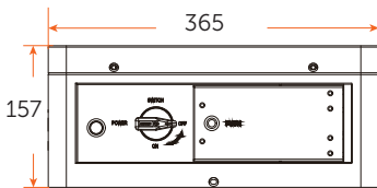
Batteriemodul (TP-HS25/TP-HS36)
