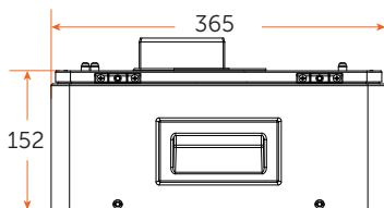
Batteriemodul (TP-HS25/TP-HS36)
