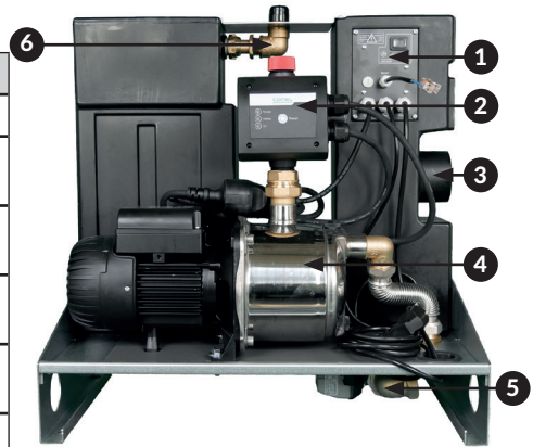
Figure 4.2.1 Conel Flow Rain-Champion Assembly
