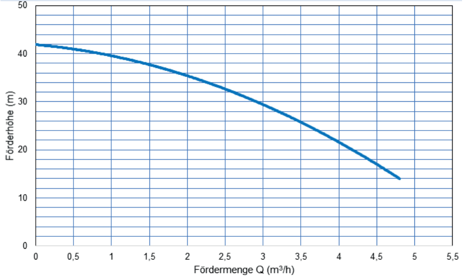
Chart 3.4.1.1 Q/H Chart Conel Flow Rain-Champion
