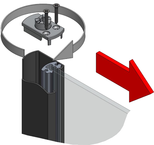
Umbau +25mm
