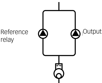
Exemplary figure of twin pumps in the solar flow with upstream flowmeter
